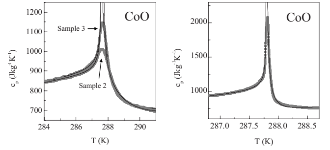
FIG. 5. Temperature dependence of c_p in close vicinity of T_N for the same three CoO crystals as in Fig. 2. On the left, the results for samples 2 and 3 are shown, whereas the results for sample 4 are shown on the right. Dots are the experimental data and the lines correspond to the best fits
