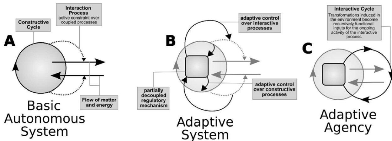
Figure 1 Conceptual diagrams of increasingly complex organizations. (a) Diagram of constitutive processes in basic autonomous systems; the constructive cycle requires a flow of matter and energy that is actively constrained by the system, giving rise to interactive processes and thus bringing about a minimal form of agency. (b) Adaptive systems show a partially decoupled mechanism that regulates interactive and constructive processes adjusting and switching between different alternatives according to external perturbations and conditions. (c) Adaptive agents appear when the interactive processes become a cycle. (Copyright © 2007 Xavier Barandiaran under a Creative Commons Attribution – Share Alike license: http://creativecommons.org/licenses/by-sa/3.0 .)
