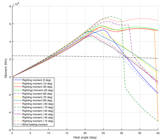
Fig. 6. Moments for the hybrid FWT-OWCs.
