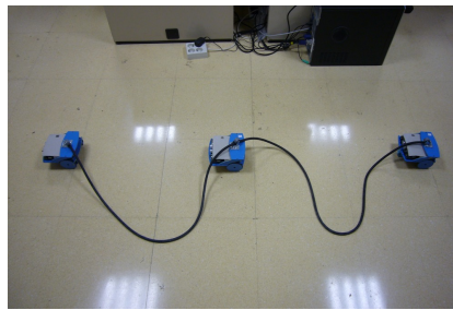
Figure 4.33: Hose-robots physical system
