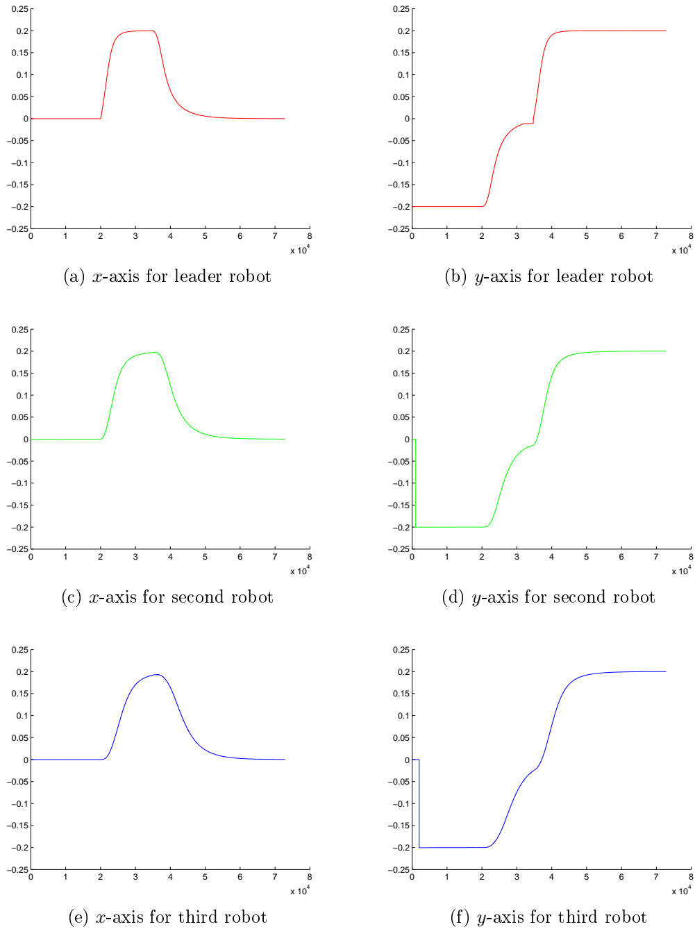
Figure 4.25: Robots velocities during the u-shaped hose transportation for the distance based heuristic f approach.
