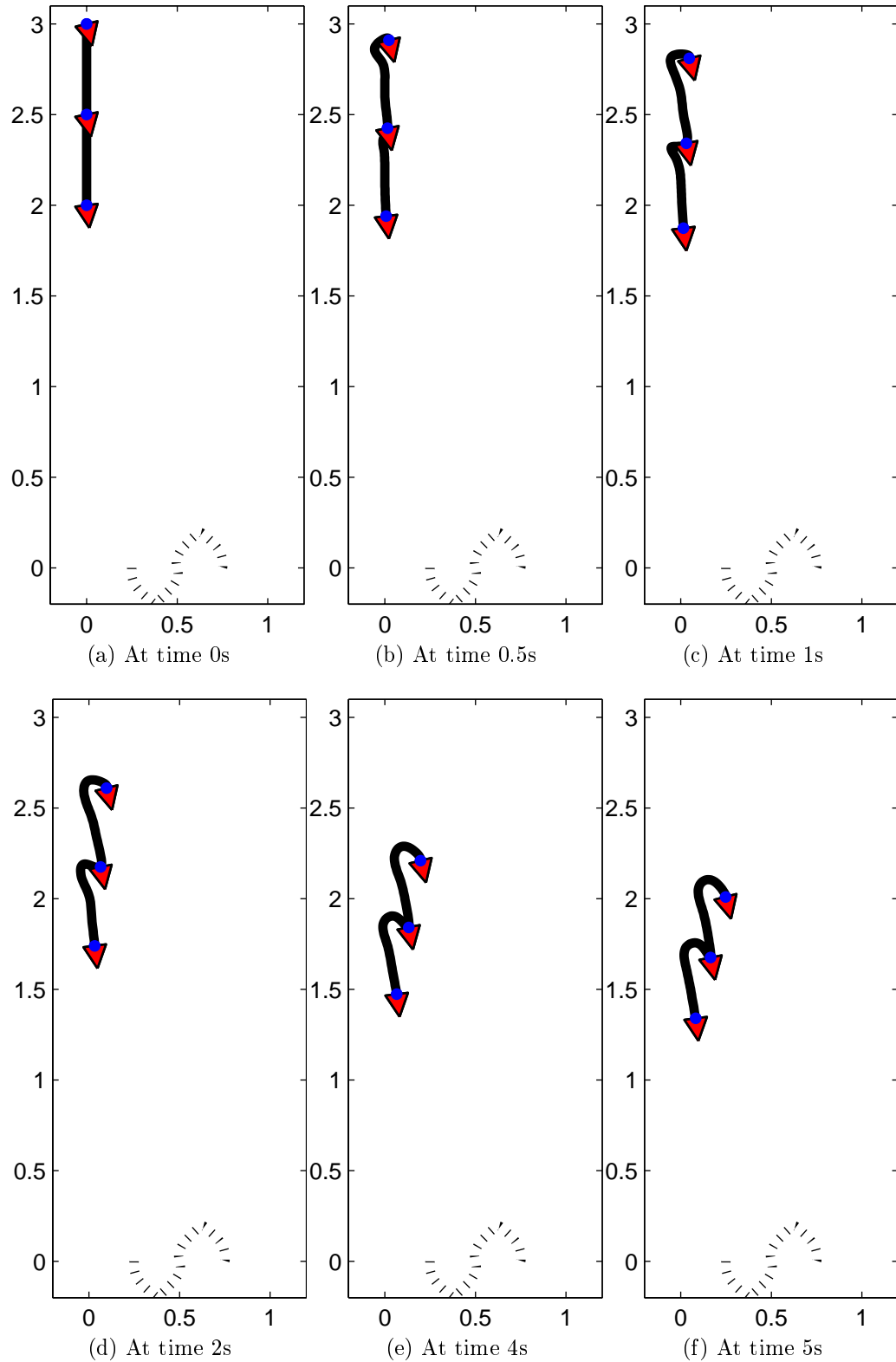
Figure 4.14: Sequence of the hose with hose internal dynamics
