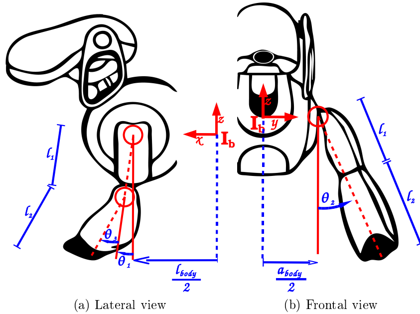
Figure 3.12: Geometry of the leg's articulations.
