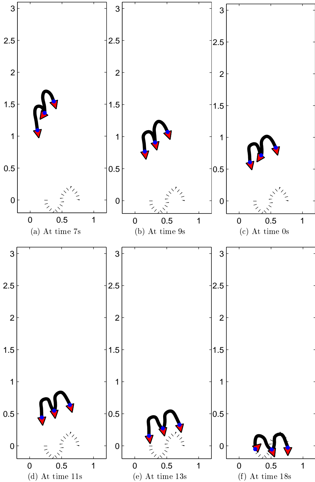
Figure 4.18: Ideal sequence of the hose with hose internal dynamics and dynamic control law(cont.)
