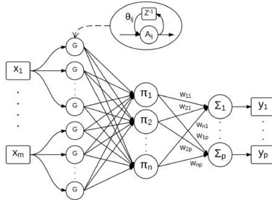
Figure 8.4: RFNN scheme.
